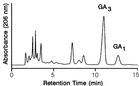
Fig. 1. Chromatogram of C_{18} HPLC of a fermentation culture (20 \mu l). Column: Spherisorb S50DS1, 25 cm \times 4.6 mm I.D. Mobile phase: 30% MeOH, containing 0.01 M H_3PO_4 adjusted with KOH to pH 3; flow-rate 1 ml/min. Detection at 206 nm, 1.0 a.u.f.s.
